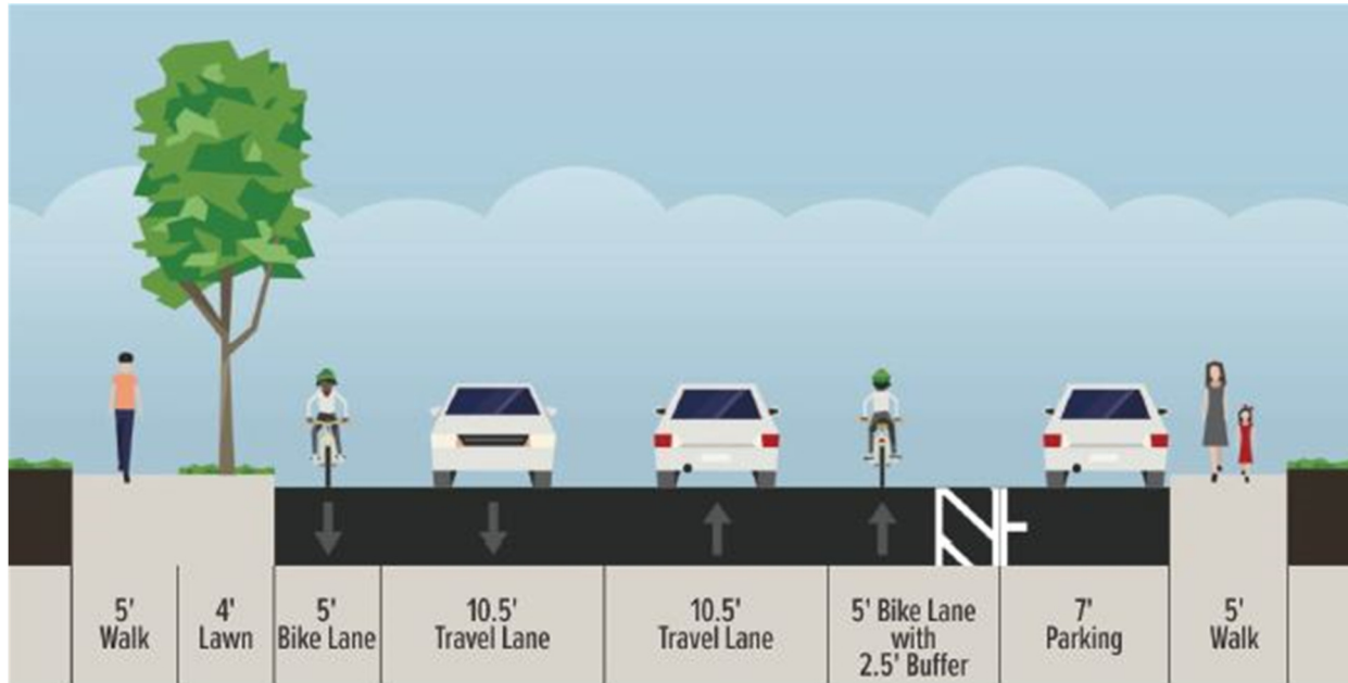
Proposed Concept for South High Street between West Broadway Street and Hovey Street
